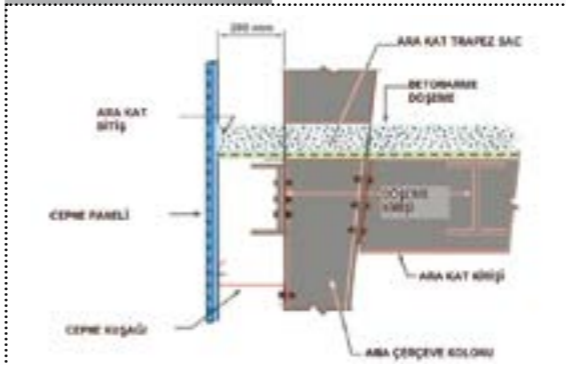
DETAILS ON THE CONNECTION BETWEEN MEZZANINE JOIST AND MAIN COLUMN
