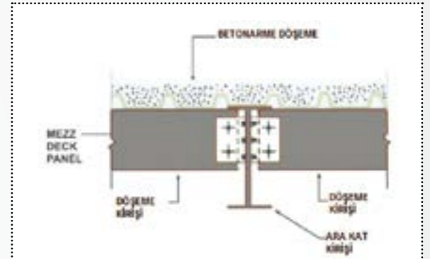
DETAILS ON THE CONNECTION BETWEEN MEZZANINE FLOORING JOIST AND MEZZANINE JOIST
